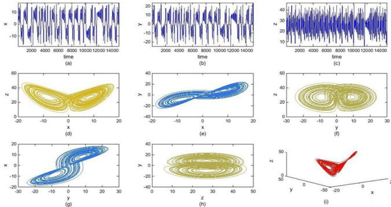
Figure 6: Simulation results of Lorenz chaotic: (a) x chaotic signal, (b) y chaotic signal and (c) z chaotic signal, (d) (x-z) attractor, (e) (x-y) attractor, (f) (y-z) attractor, (g) (y-x) attractor, (h) (z-y) attractor, (i) (x-y-z) attractor.
