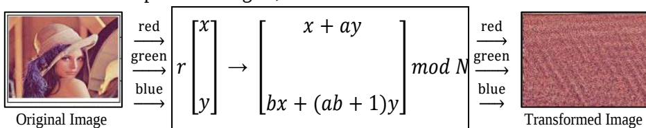
Figure 1: Arnold cat map implementation
