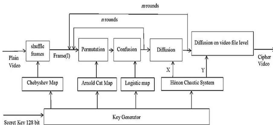
Figure 7: The architecture and the methodology of the proposed encryption
