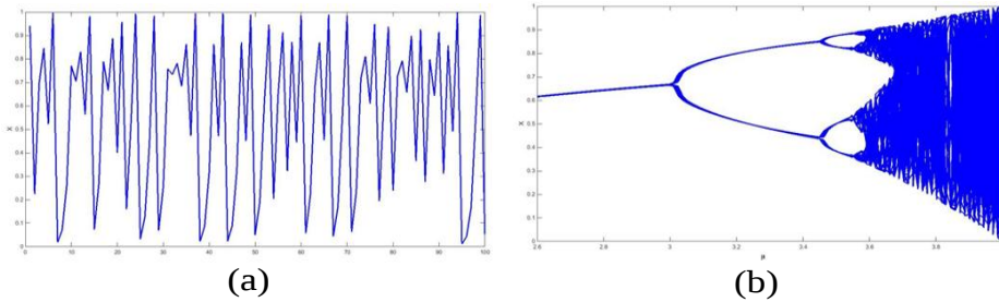
Figure 2: (a) Attractors for the Logistic Map with \mu=3.99 . (b) Bifurcation Diagram for the Logistic Map
