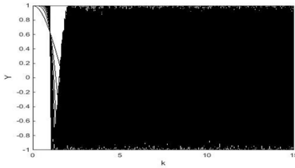
Figure 4: Bifurcation diagram of the chaotic Chepyshev map at x_0=0.02 .
