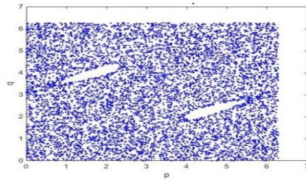
Figure 5: Attractors for the chaotic Standard map with c=4.6 and p=0.666 and q=0.282 .
